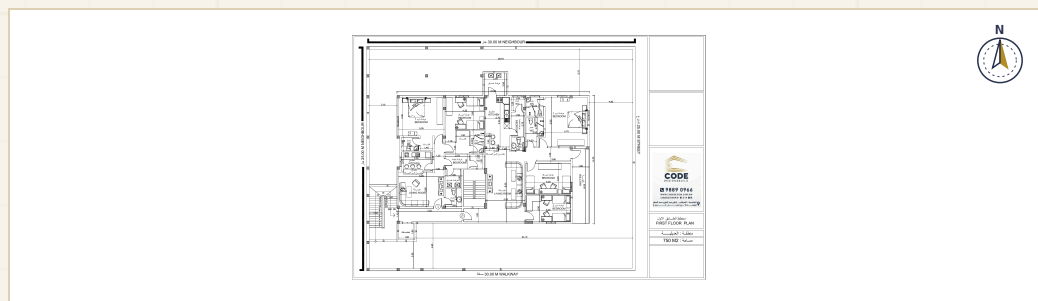
Furnished first floor plan
