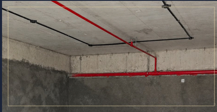
11 Overhead service installation
